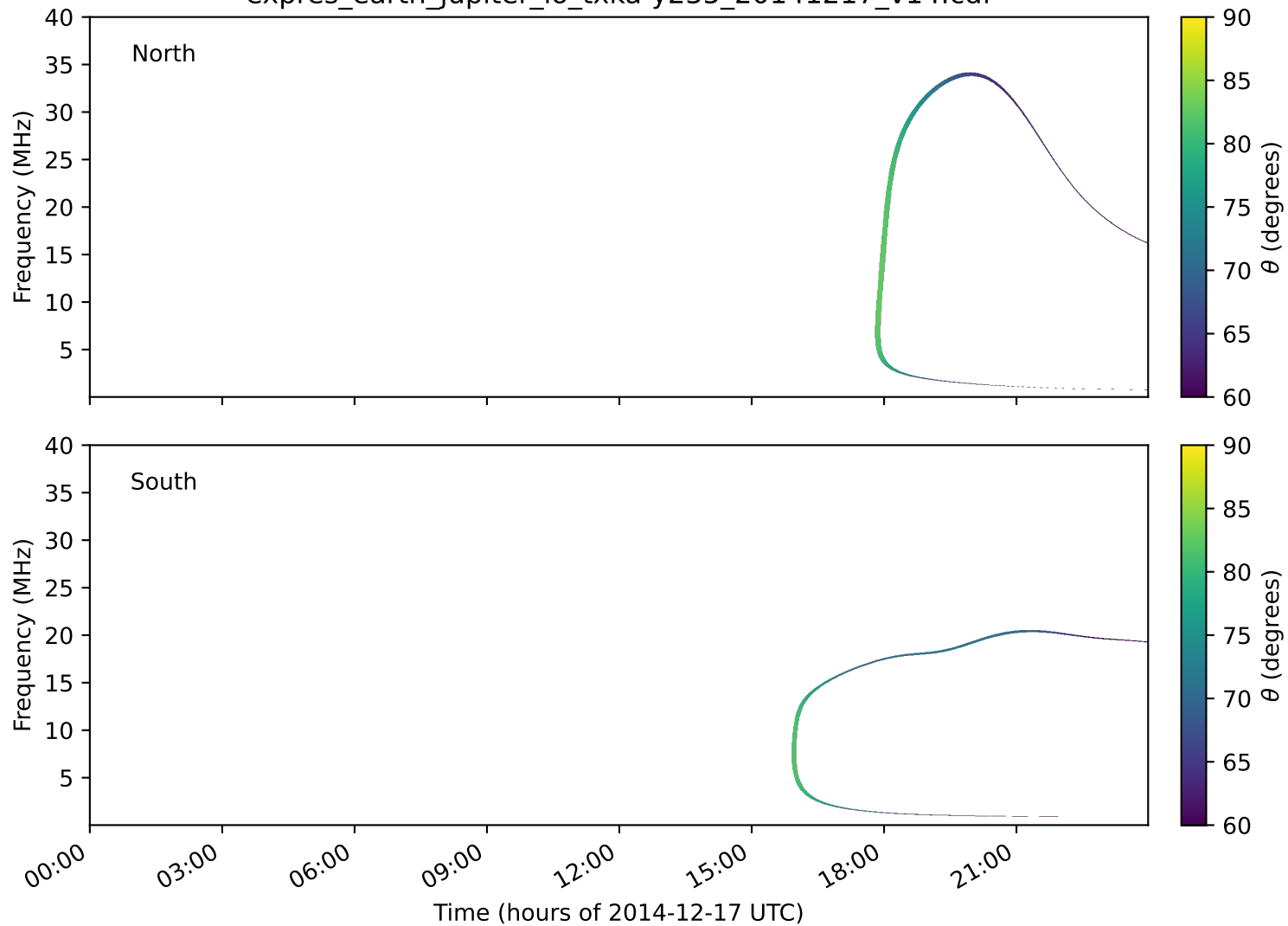
expres_earth_jupiter_io_txka-y235_20141217_v14.cdf
