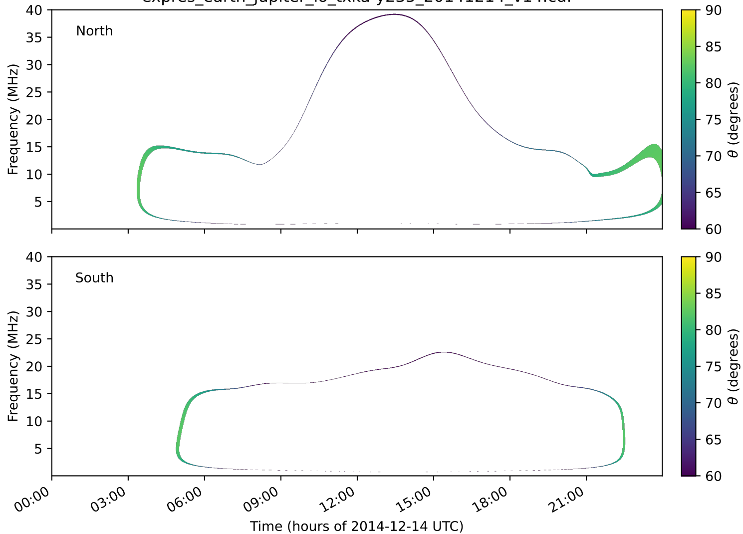
expres_earth_jupiter_io_txka-y235_20141214_v14.cdf
