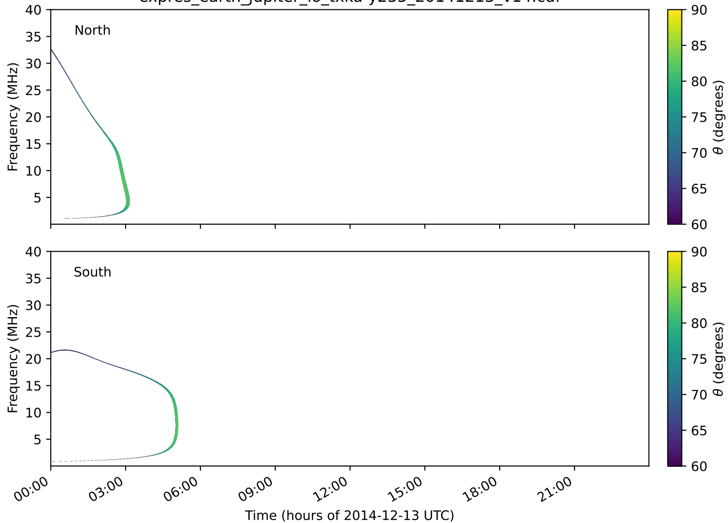
expres_earth_jupiter_io_txka-y235_20141213_v14.cdf
