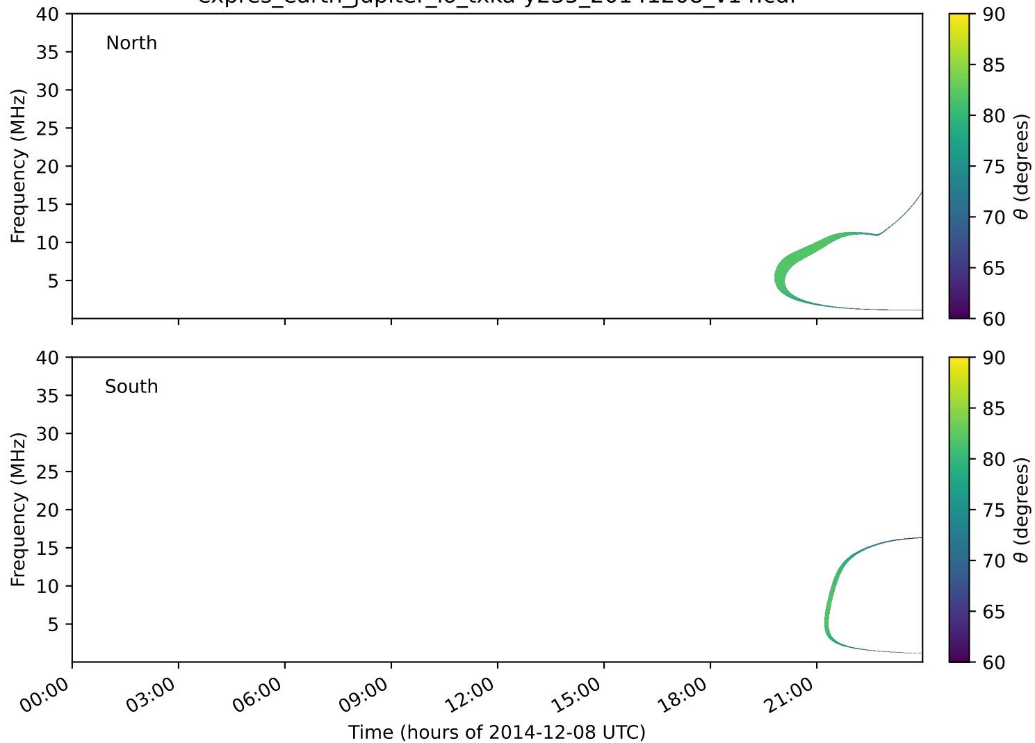
expres_earth_jupiter_io_txka-y235_20141208_v14.cdf
