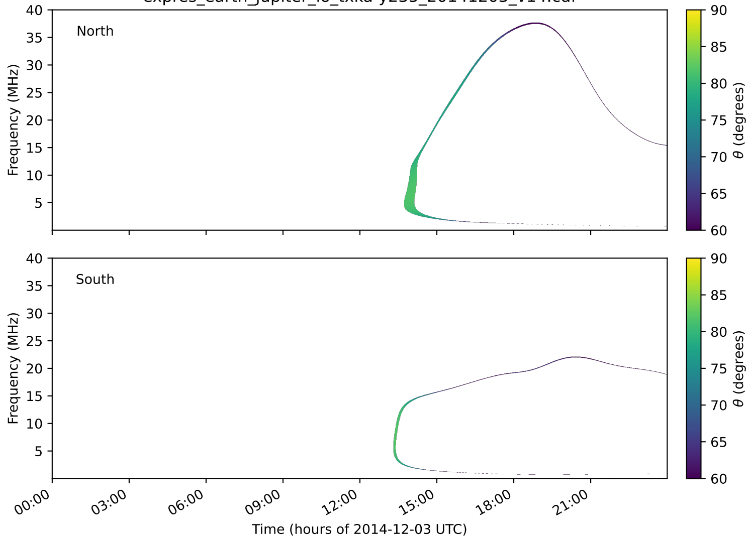
expres_earth_jupiter_io_txka-y235_20141203_v14.cdf
