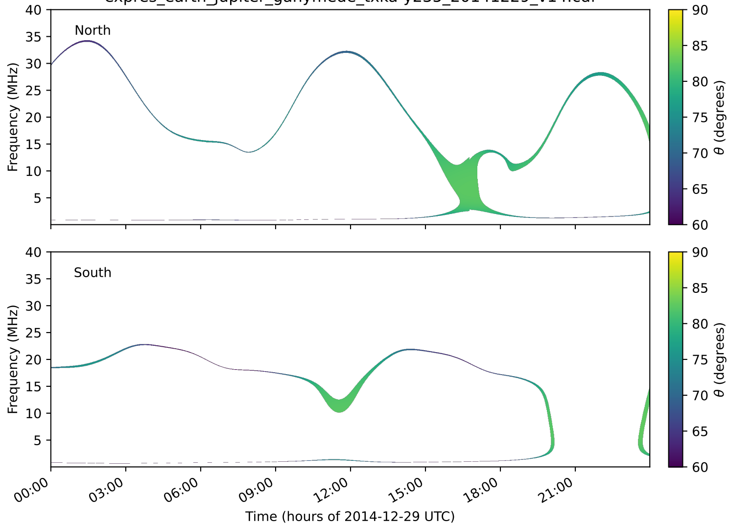
expres_earth_jupiter_ganymede_txka-y235_20141229_v14.cdf
