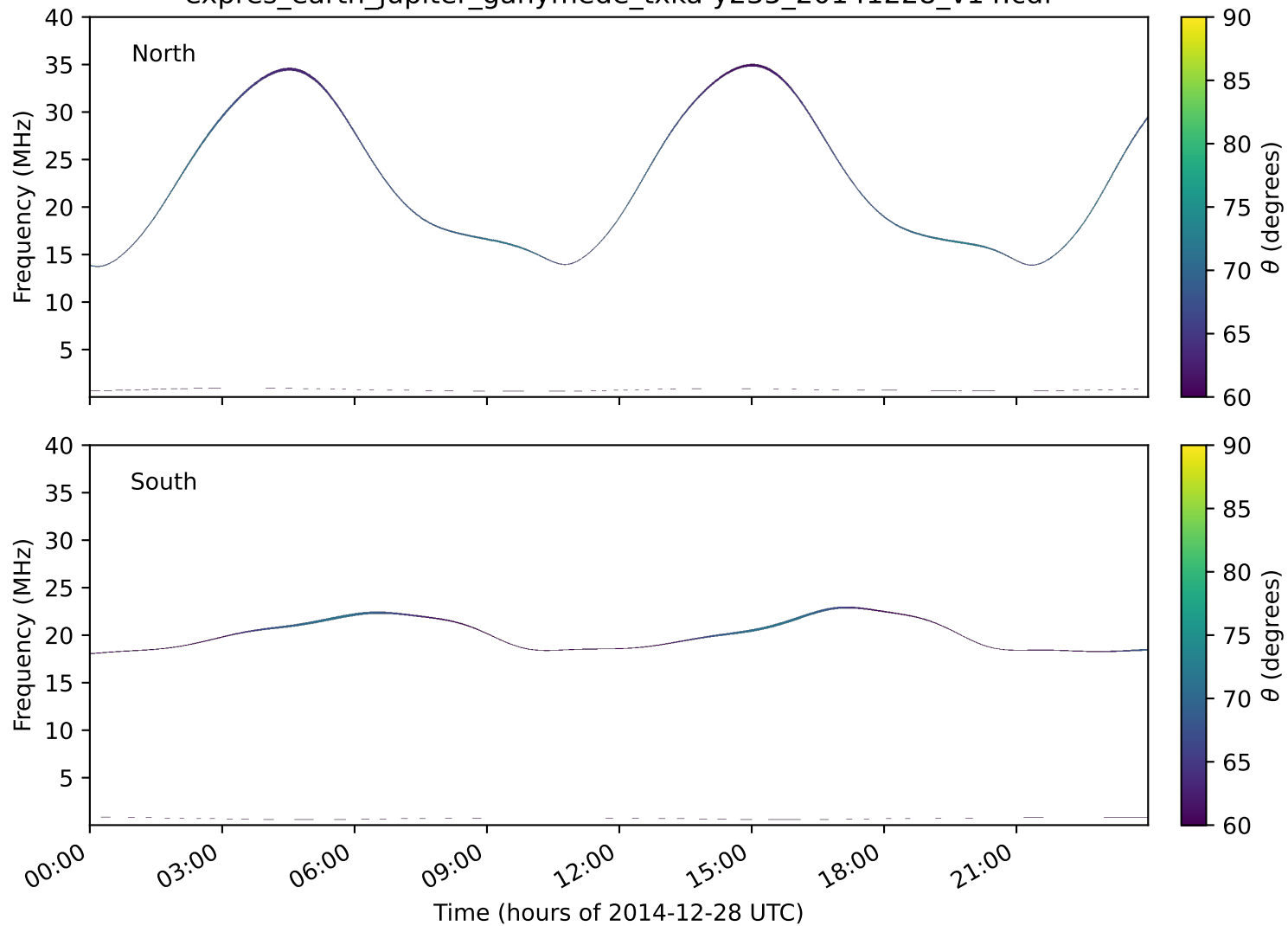
expres_earth_jupiter_ganymede_txka-y235_20141228_v14.cdf
