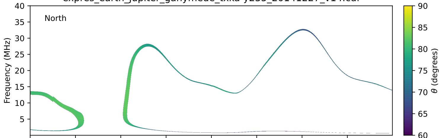
expres_earth_jupiter_ganymede_txka-y235_20141227_v14.cdf
