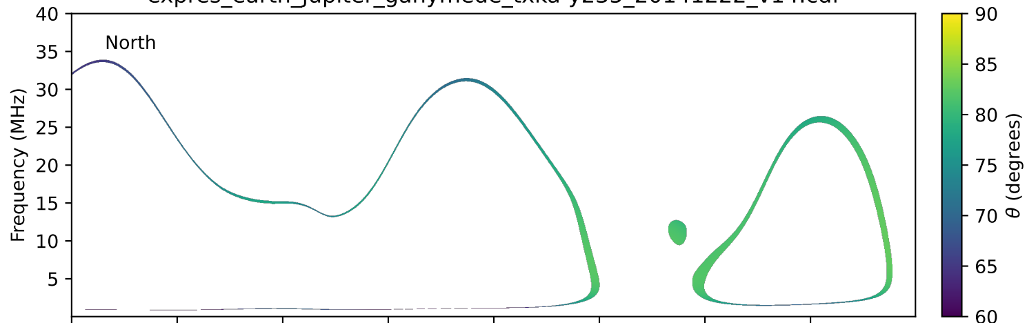
expres_earth_jupiter_ganymede_txka-y235_20141222_v14.cdf
