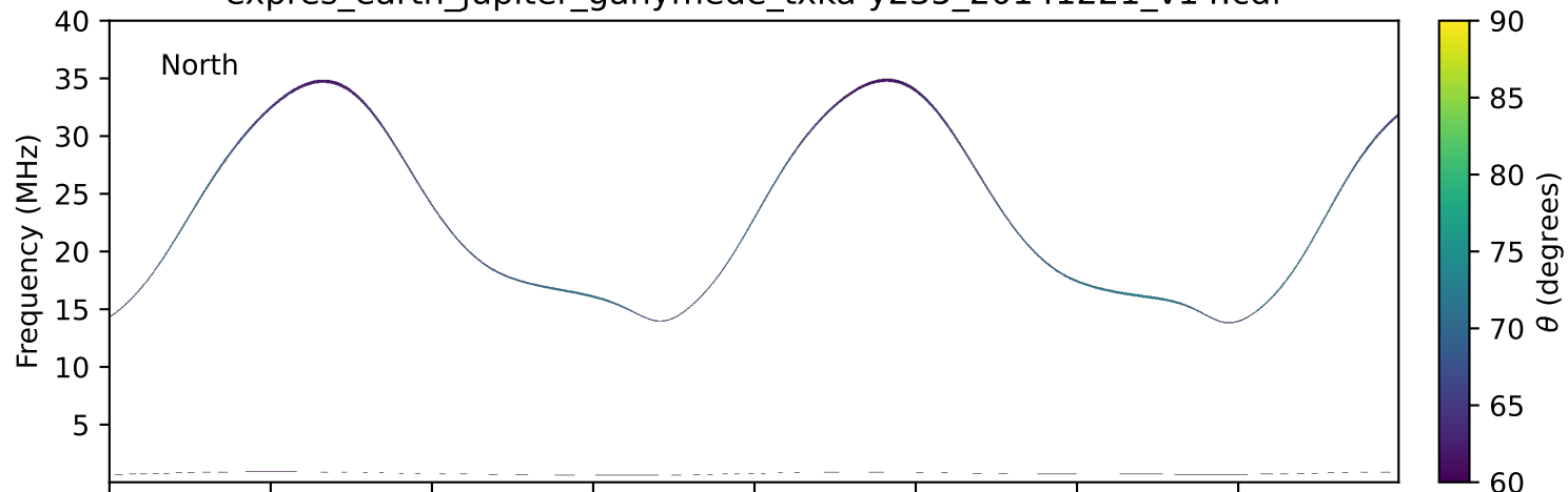
expres_earth_jupiter_ganymede_txka-y235_20141221_v14.cdf
