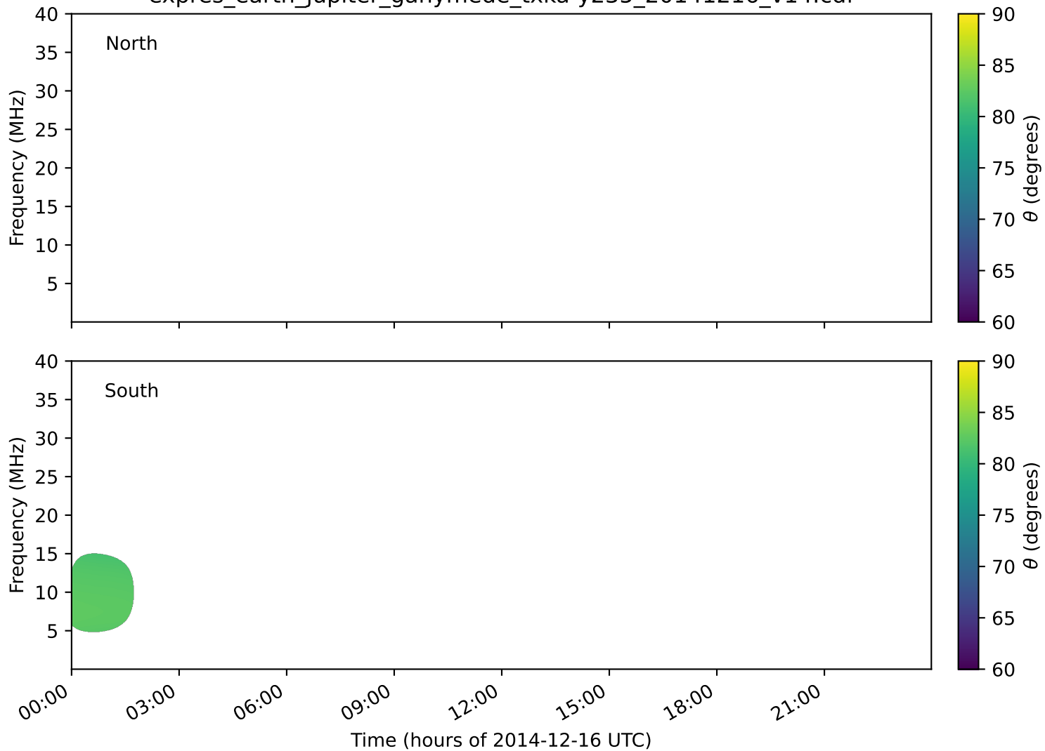
expres_earth_jupiter_ganymede_txka-y235_20141216_v14.cdf
