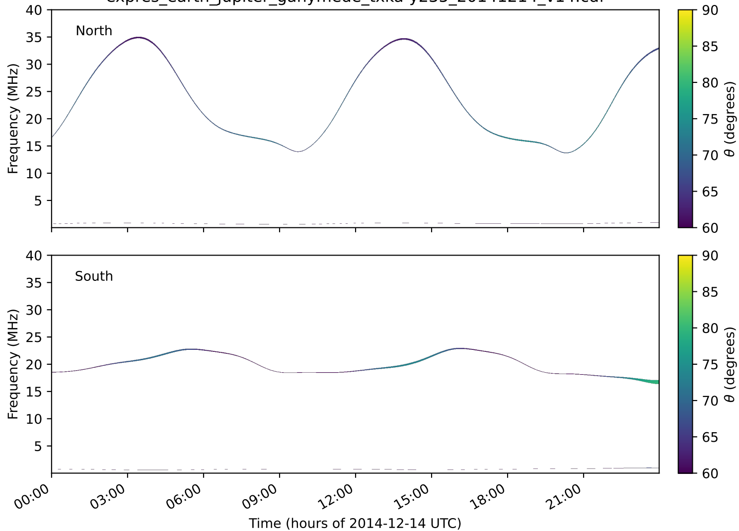
expres_earth_jupiter_ganymede_txka-y235_20141214_v14.cdf
