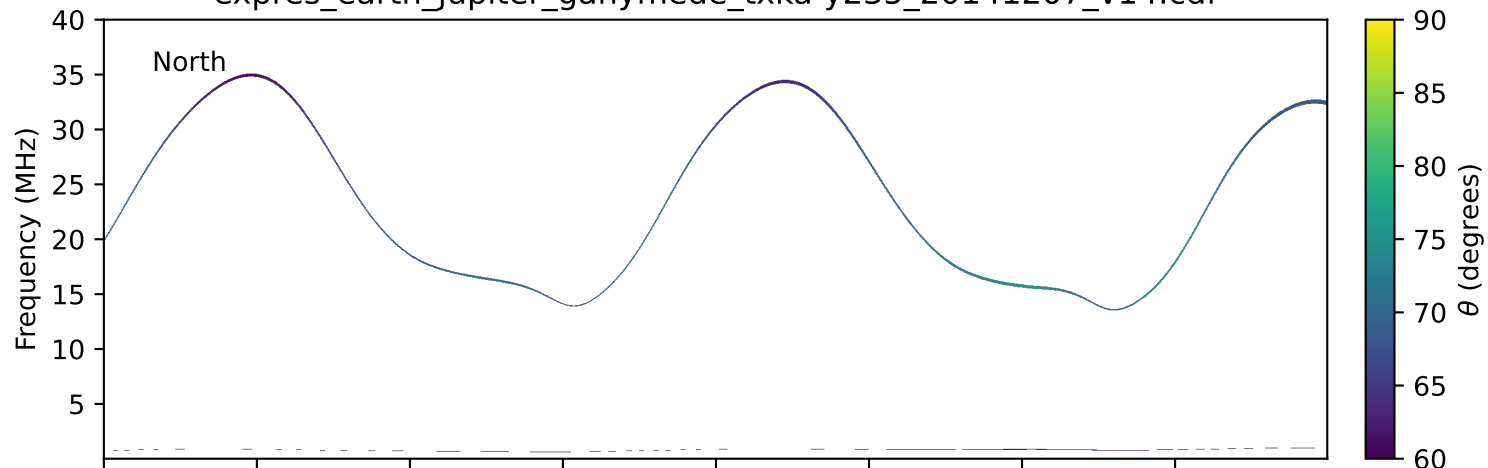
expres_earth_jupiter_ganymede_txka-y235_20141207_v14.cdf
