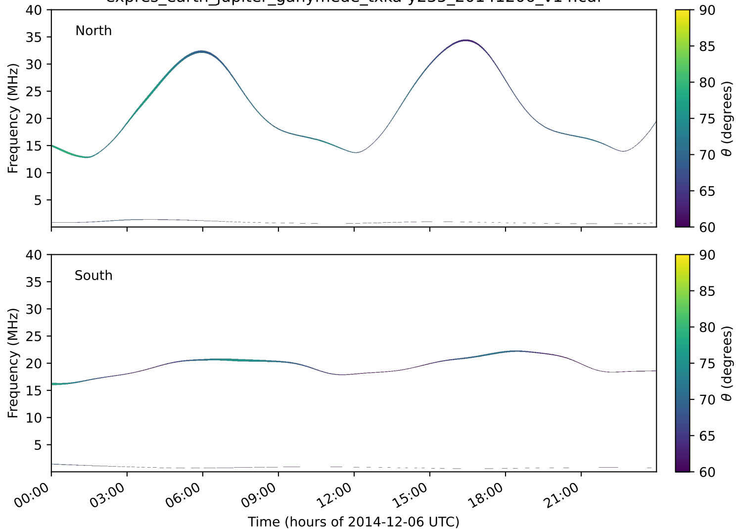
expres_earth_jupiter_ganymede_txka-y235_20141206_v14.cdf
