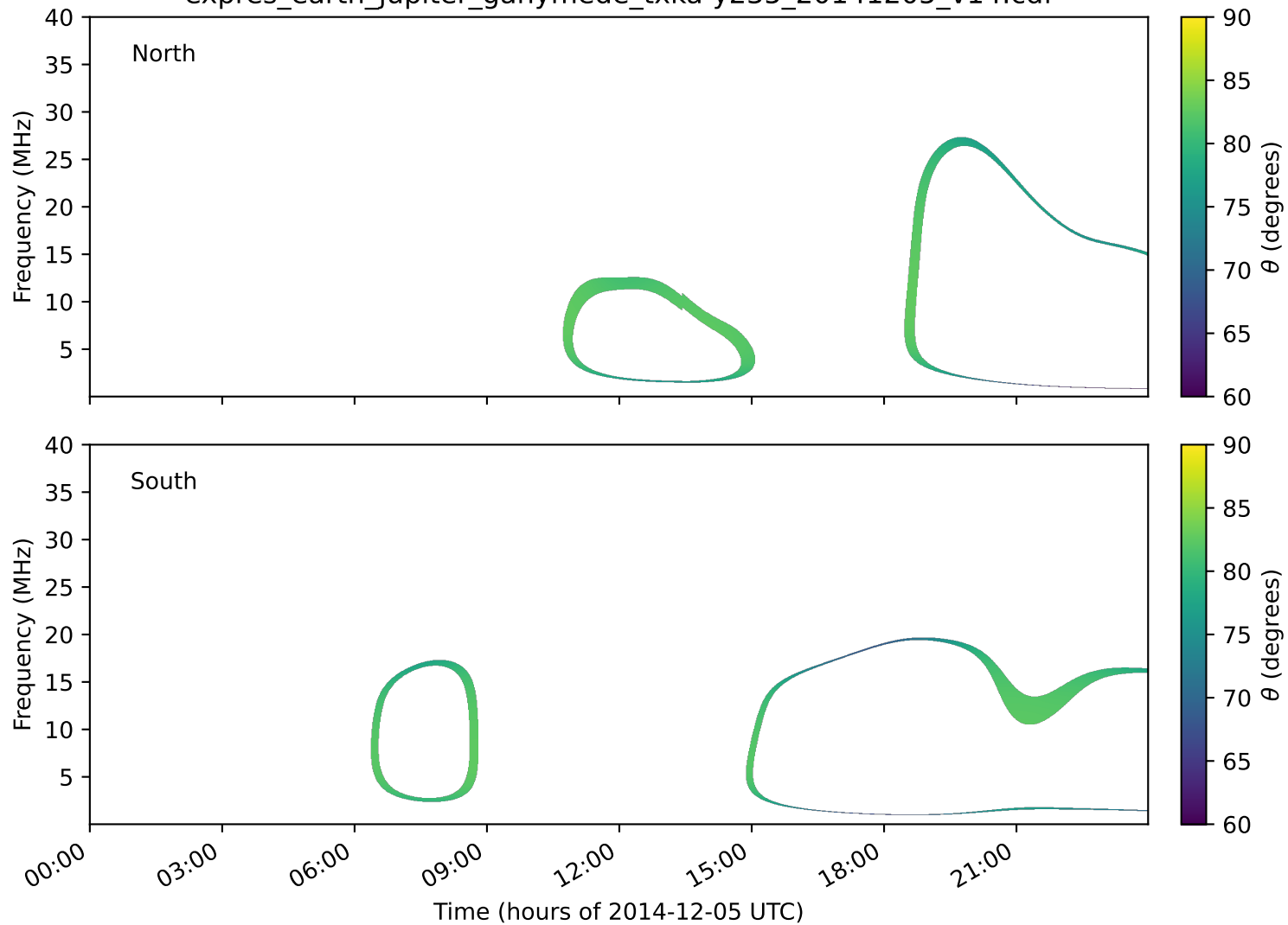
expres_earth_jupiter_ganymede_txka-y235_20141205_v14.cdf
