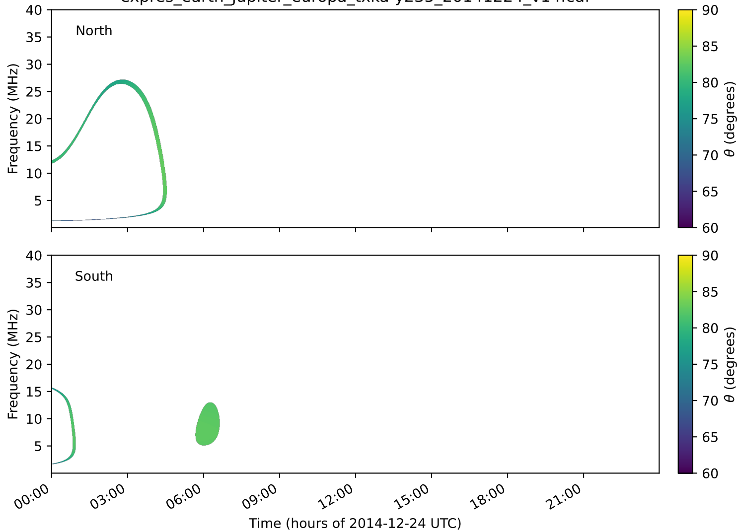
expres_earth_jupiter_europa_txka-y235_20141224_v14.cdf
