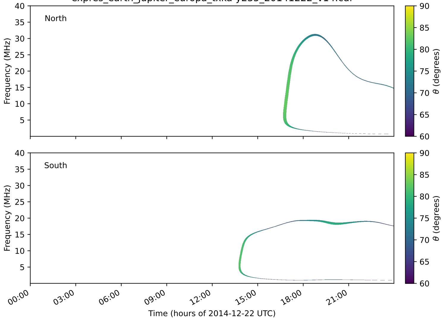
expres_earth_jupiter_europa_txka-y235_20141222_v14.cdf
