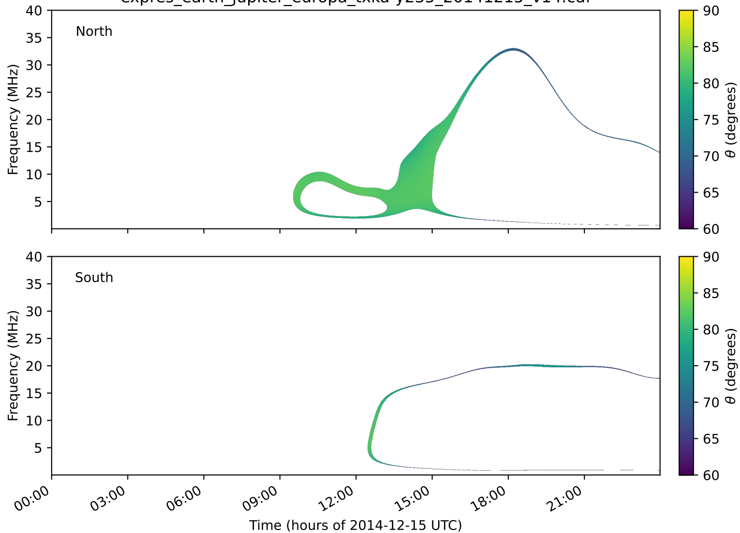
expres_earth_jupiter_europa_txka-y235_20141215_v14.cdf
