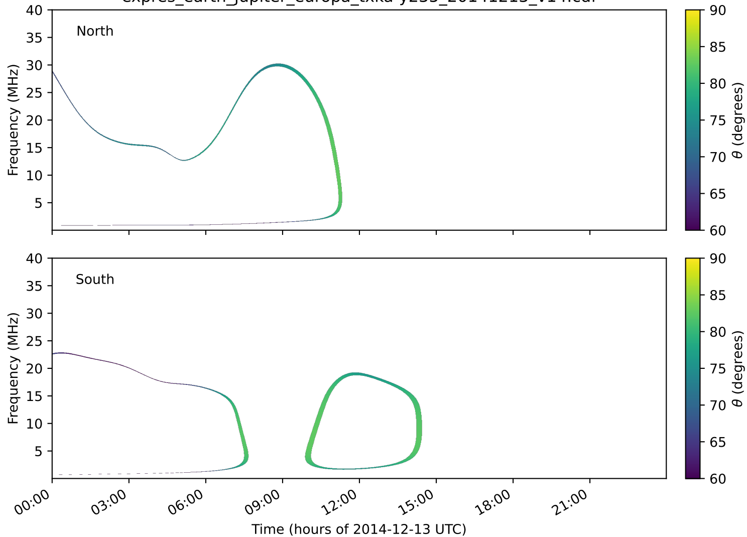
expres_earth_jupiter_europa_txka-y235_20141213_v14.cdf
