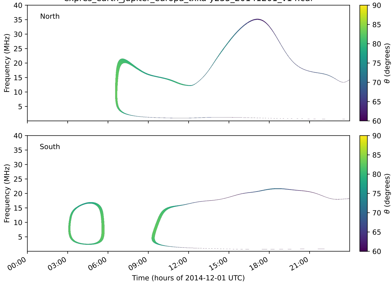
expres_earth_jupiter_europa_txka-y235_20141201_v14.cdf
