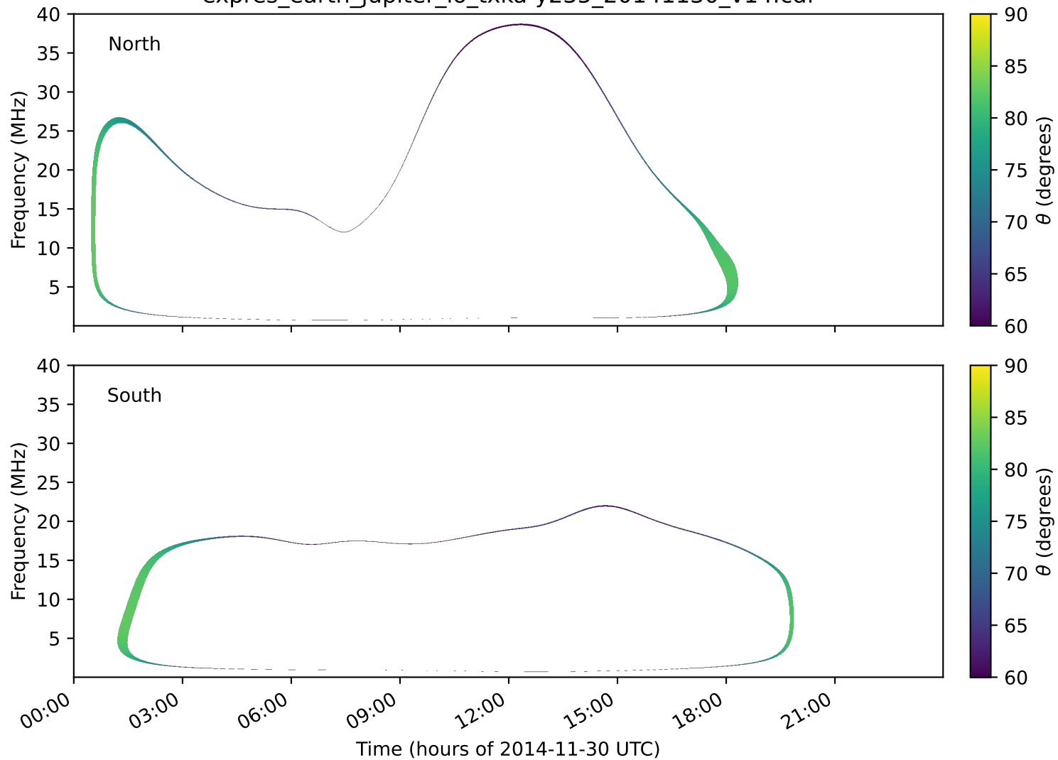
expres_earth_jupiter_io_txka-y235_20141130_v14.cdf
