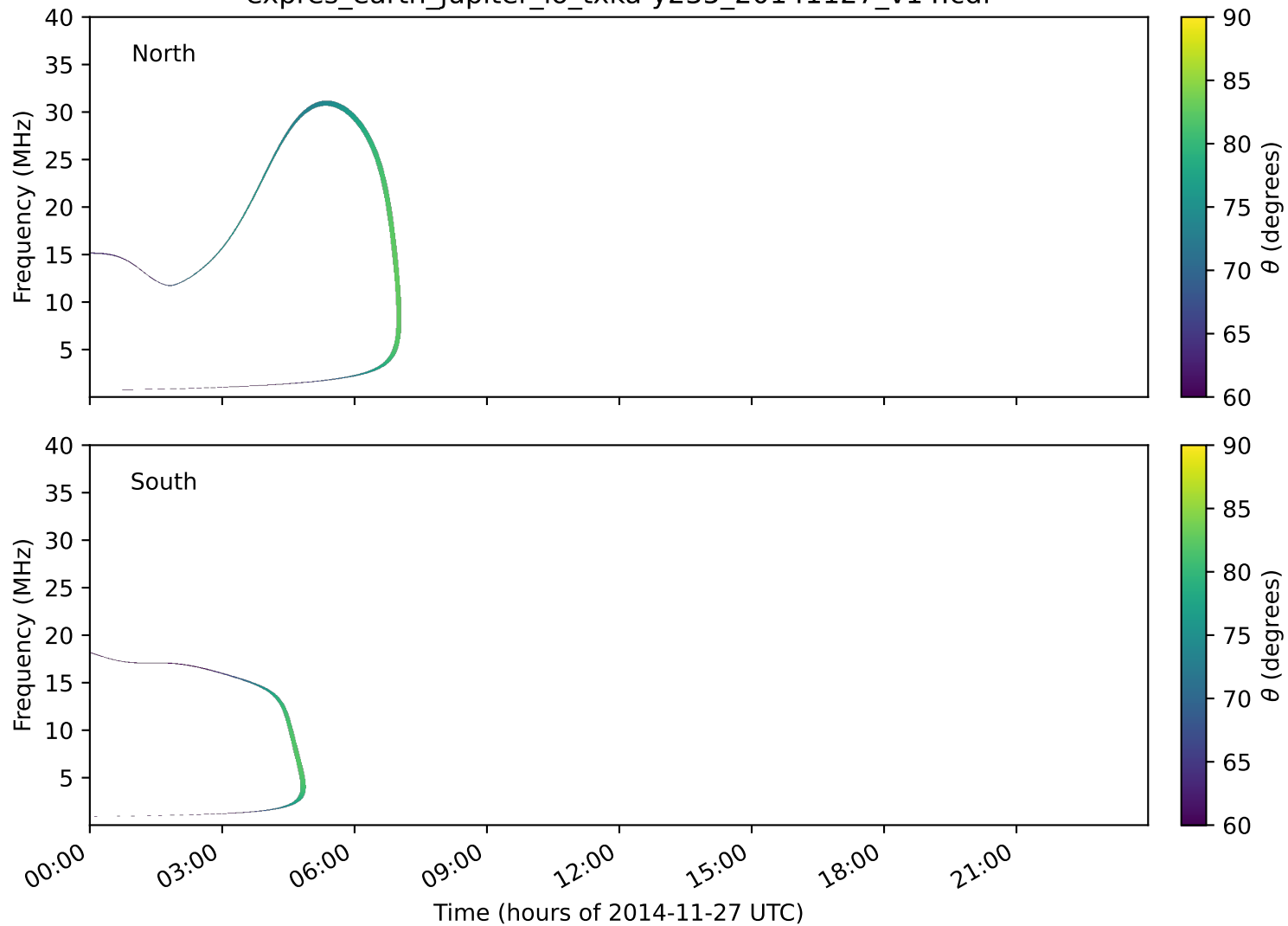
expres_earth_jupiter_io_txka-y235_20141127_v14.cdf
