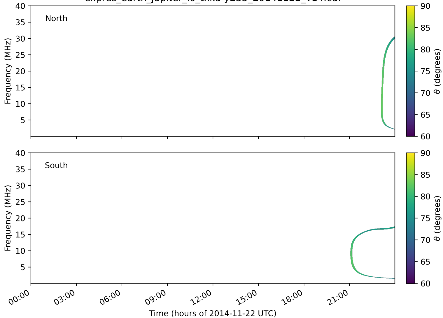
expres_earth_jupiter_io_txka-y235_20141122_v14.cdf
