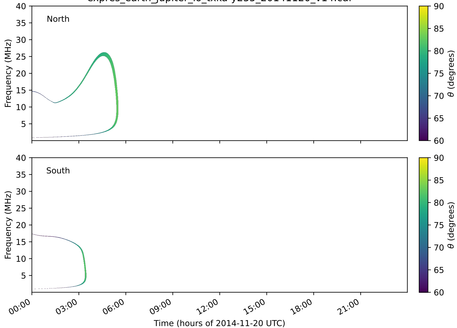
expres_earth_jupiter_io_txka-y235_20141120_v14.cdf
