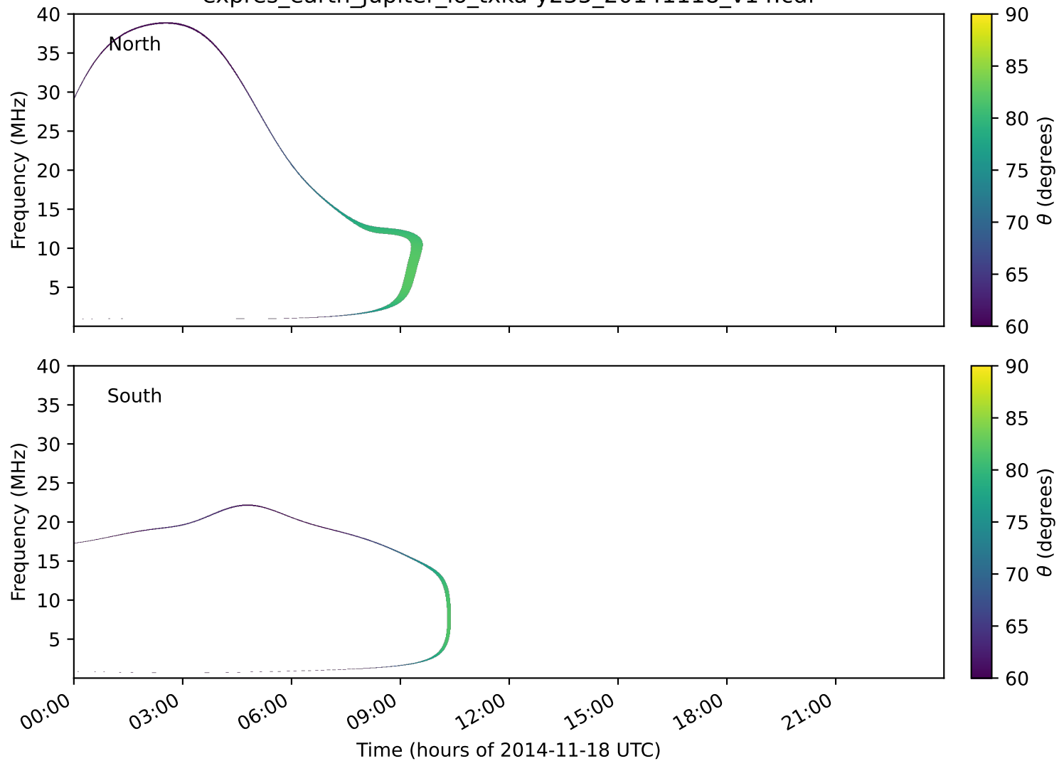
expres_earth_jupiter_io_txka-y235_20141118_v14.cdf
