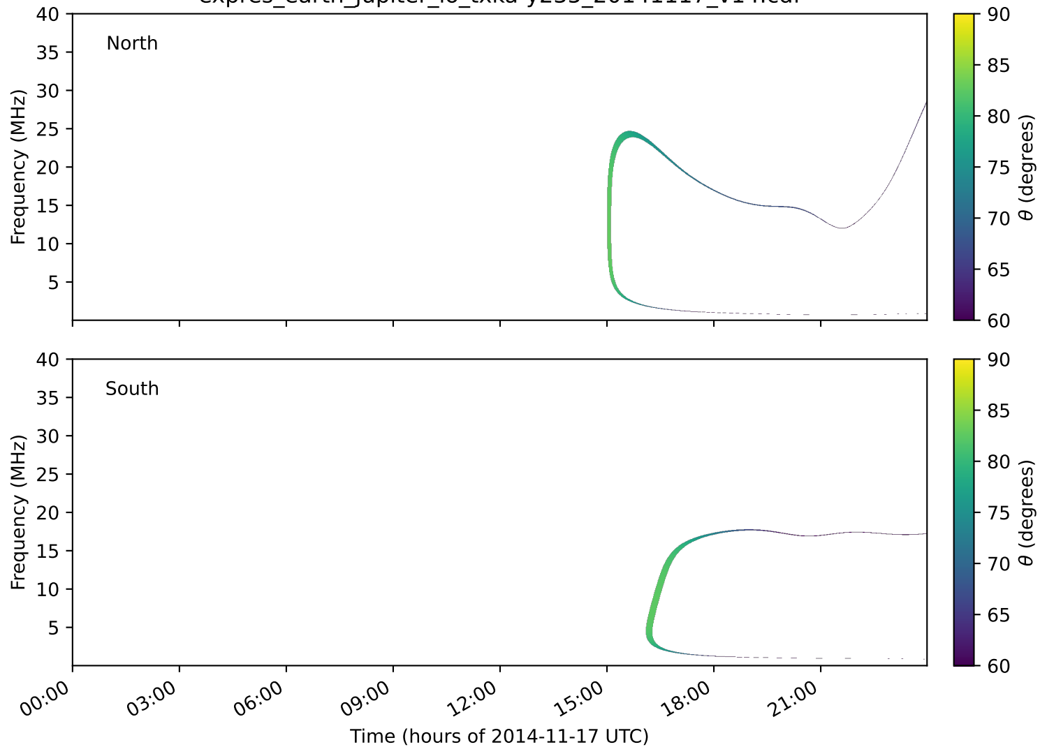
expres_earth_jupiter_io_txka-y235_20141117_v14.cdf
