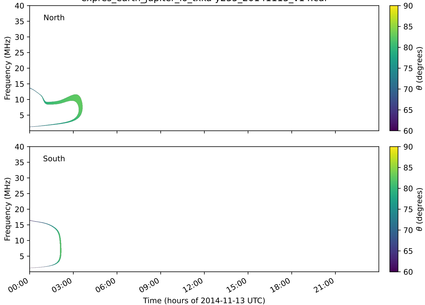
expres_earth_jupiter_io_txka-y235_20141113_v14.cdf
