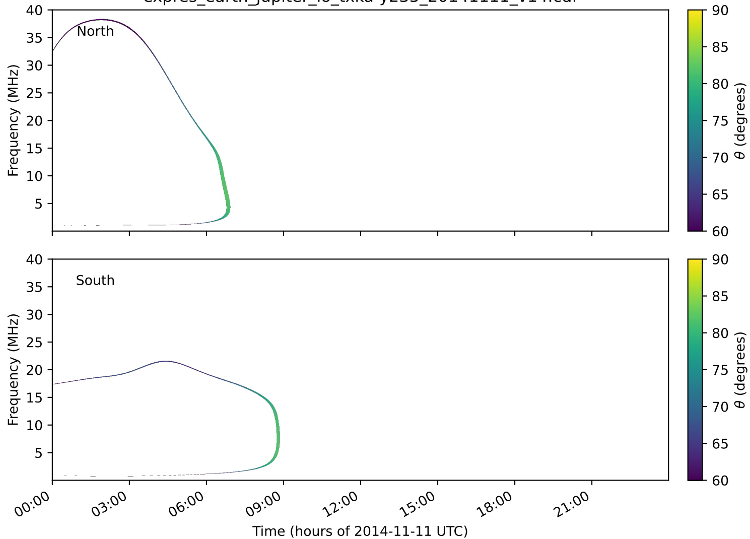
expres_earth_jupiter_io_txka-y235_20141111_v14.cdf
