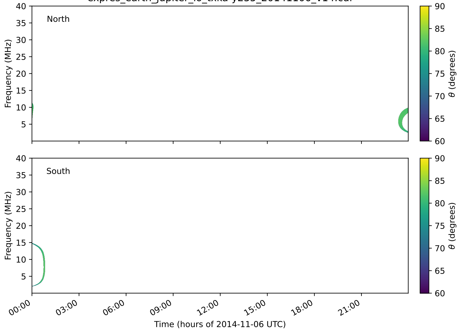
expres_earth_jupiter_io_txka-y235_20141106_v14.cdf
