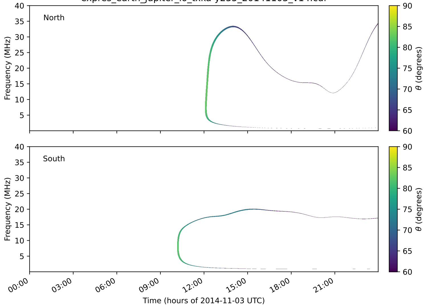
expres_earth_jupiter_io_txka-y235_20141103_v14.cdf
