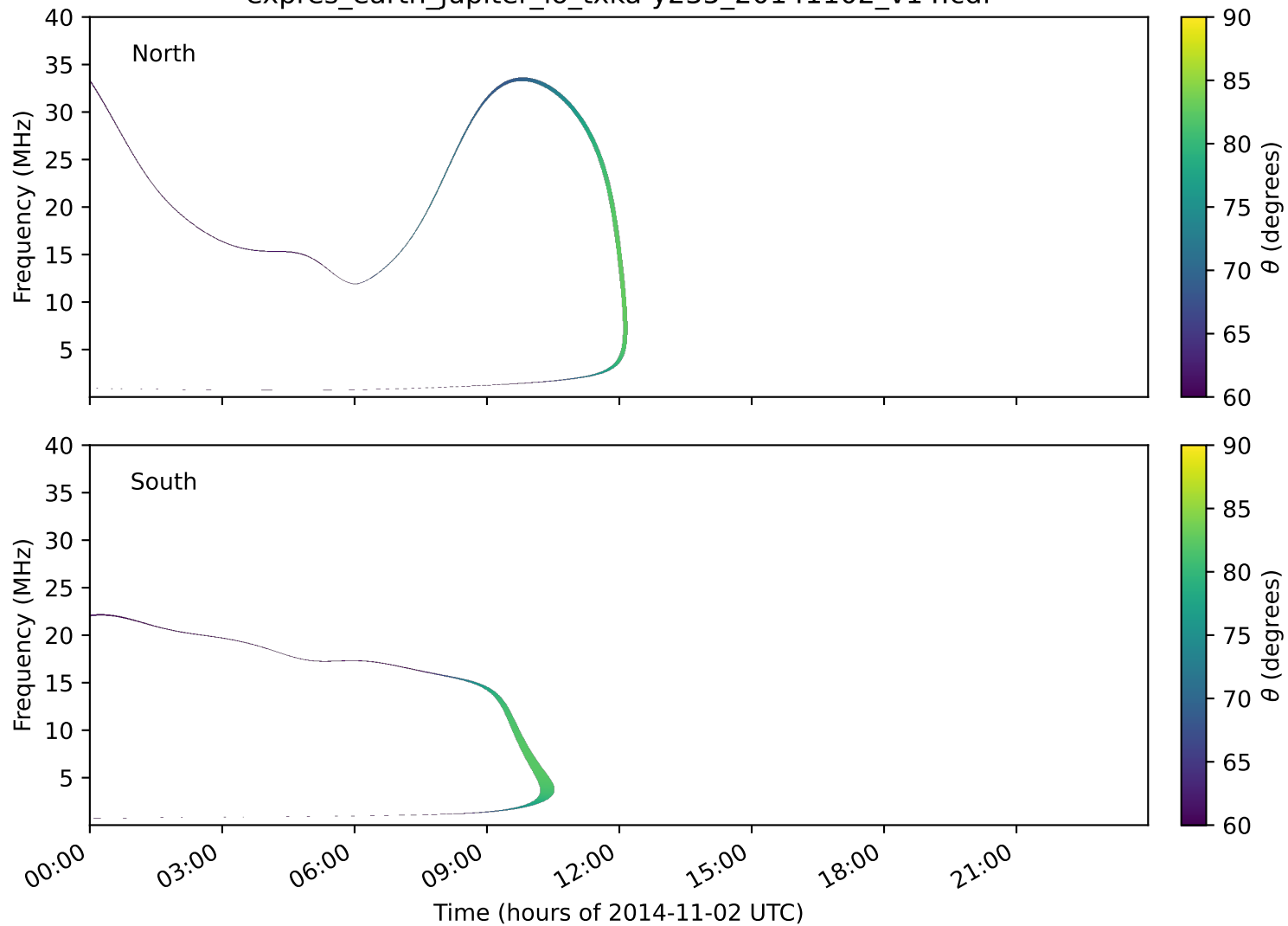
expres_earth_jupiter_io_txka-y235_20141102_v14.cdf
