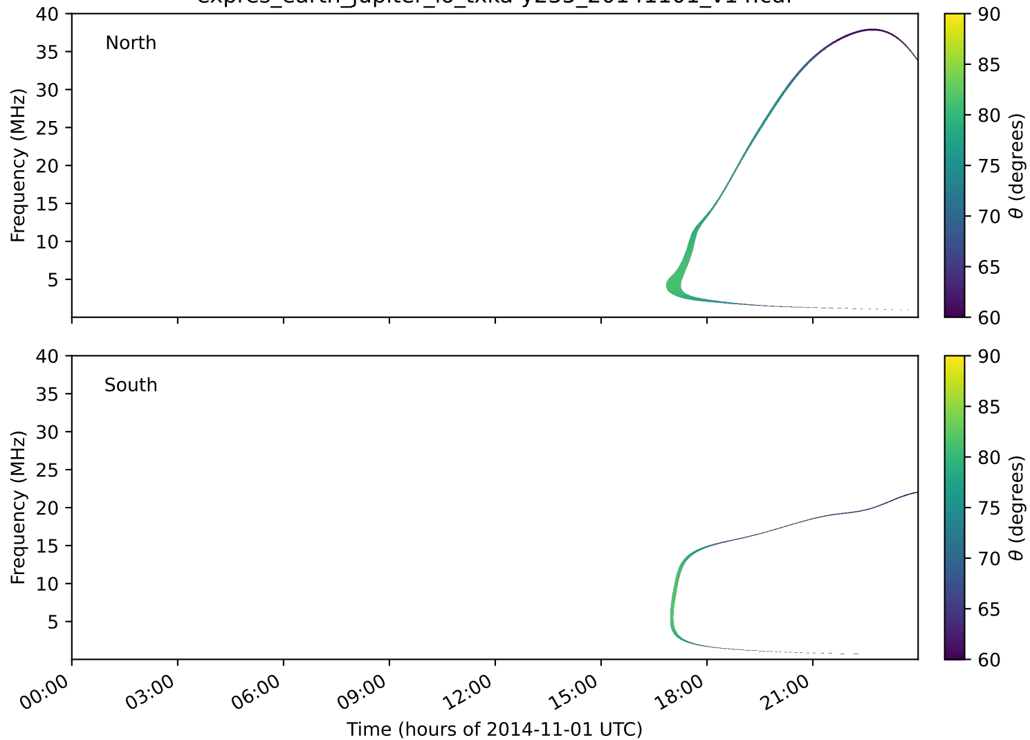
expres_earth_jupiter_io_txka-y235_20141101_v14.cdf
