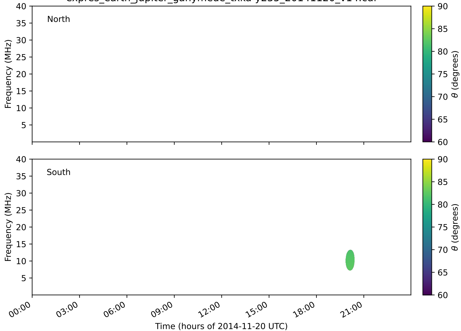
expres_earth_jupiter_ganymede_txka-y235_20141120_v14.cdf
