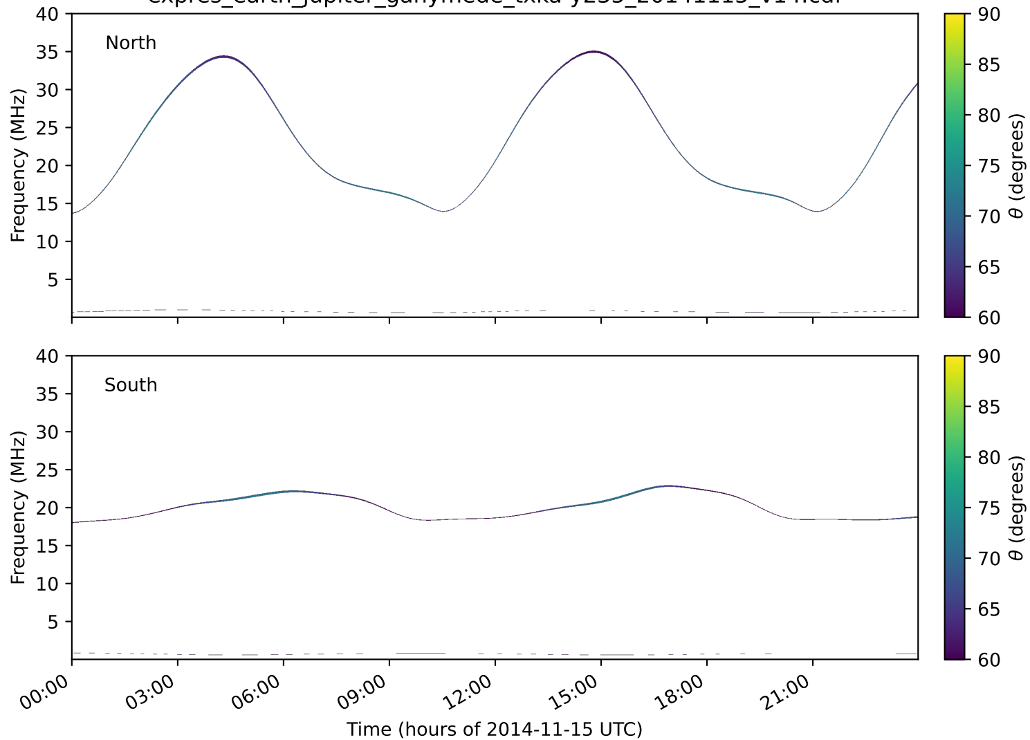
expres_earth_jupiter_ganymede_txka-y235_20141115_v14.cdf
