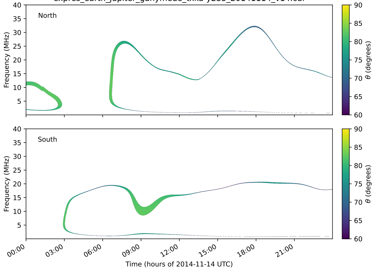
expres_earth_jupiter_ganymede_txka-y235_20141114_v14.cdf
