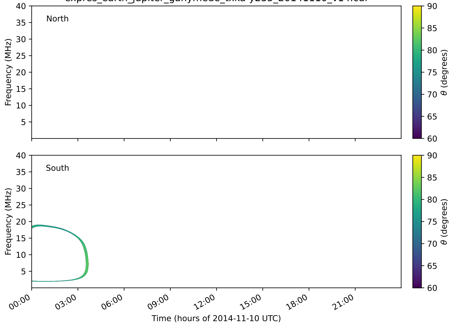
expres_earth_jupiter_ganymede_txka-y235_20141110_v14.cdf
