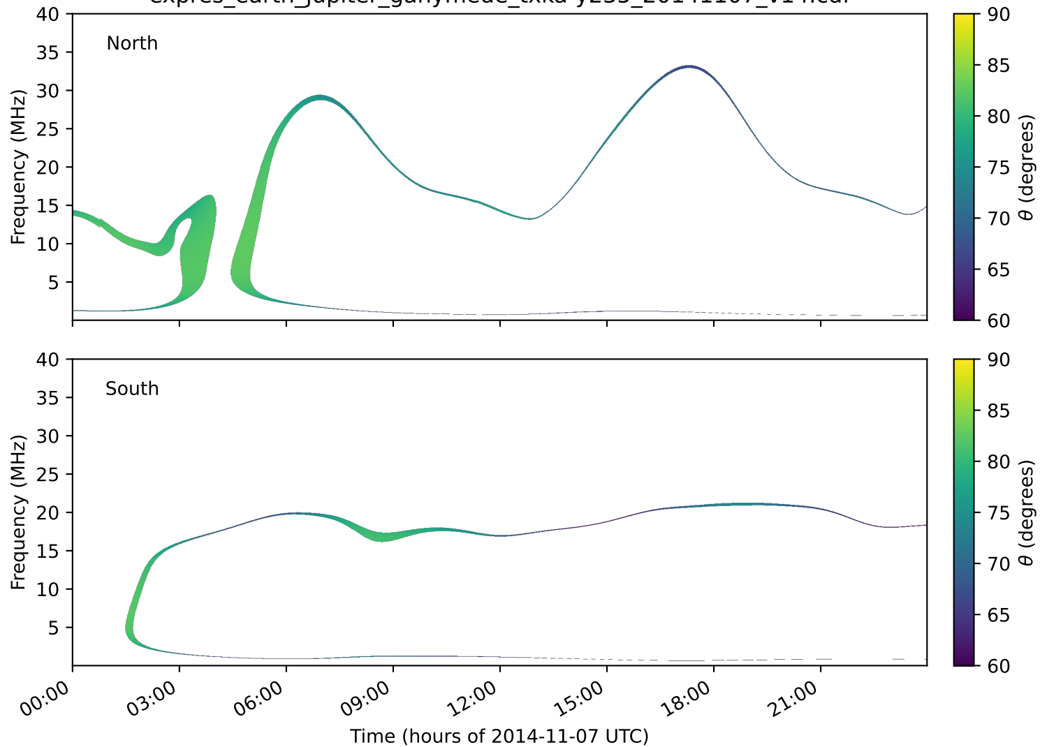
expres_earth_jupiter_ganymede_txka-y235_20141107_v14.cdf
