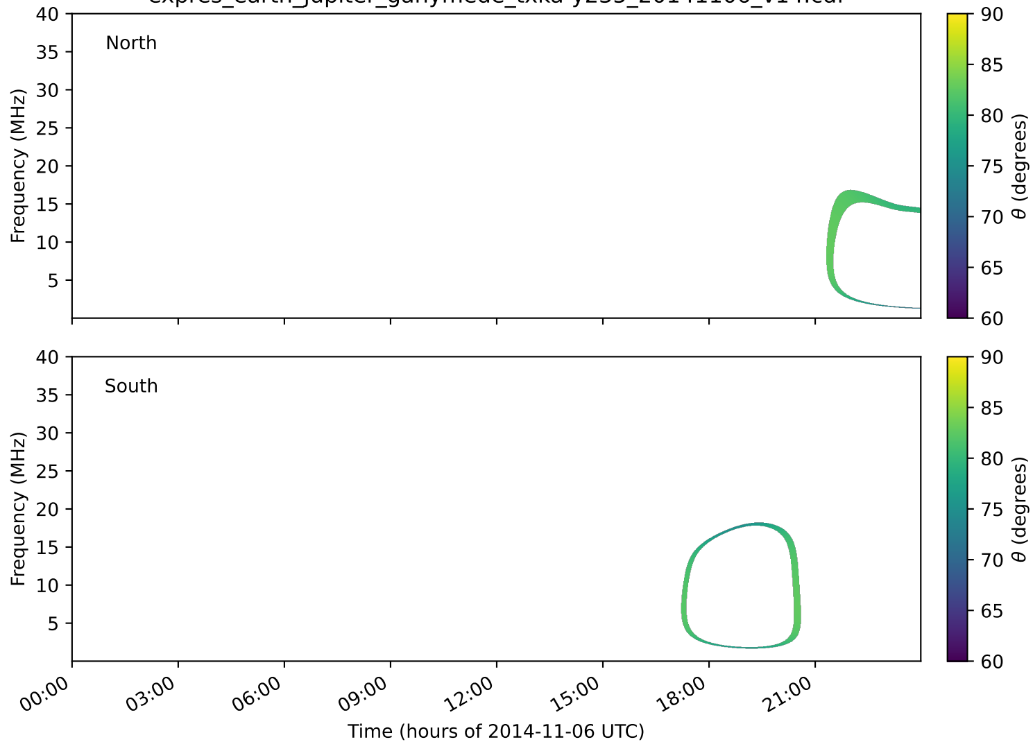
expres_earth_jupiter_ganymede_txka-y235_20141106_v14.cdf
