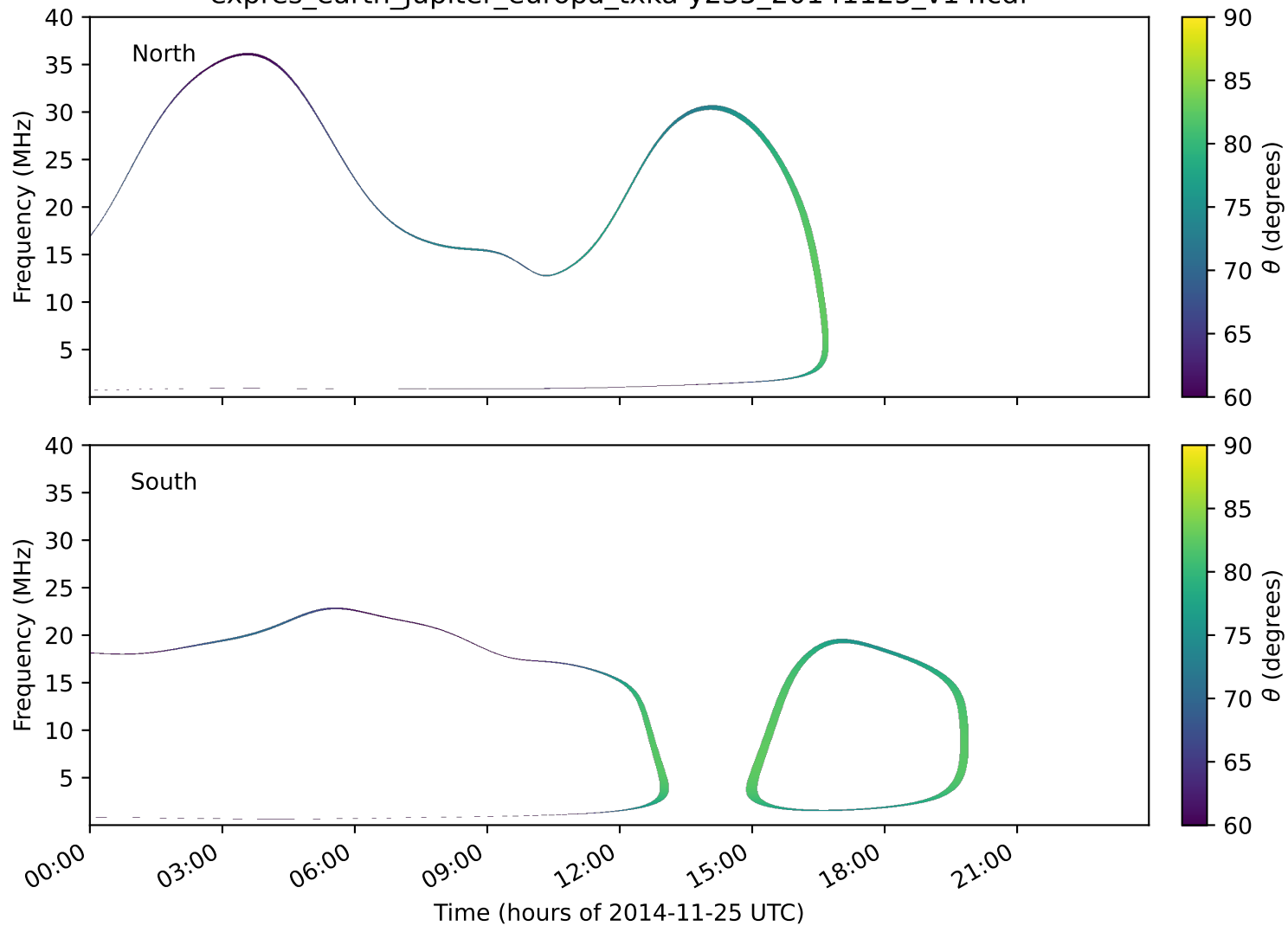
expres_earth_jupiter_europa_txka-y235_20141125_v14.cdf
