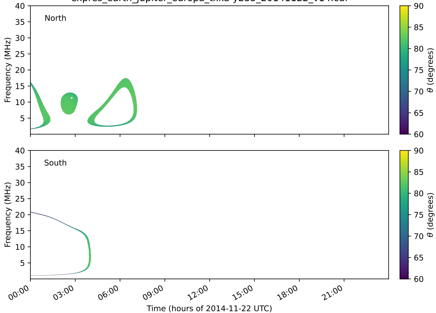
expres_earth_jupiter_europa_txka-y235_20141122_v14.cdf
