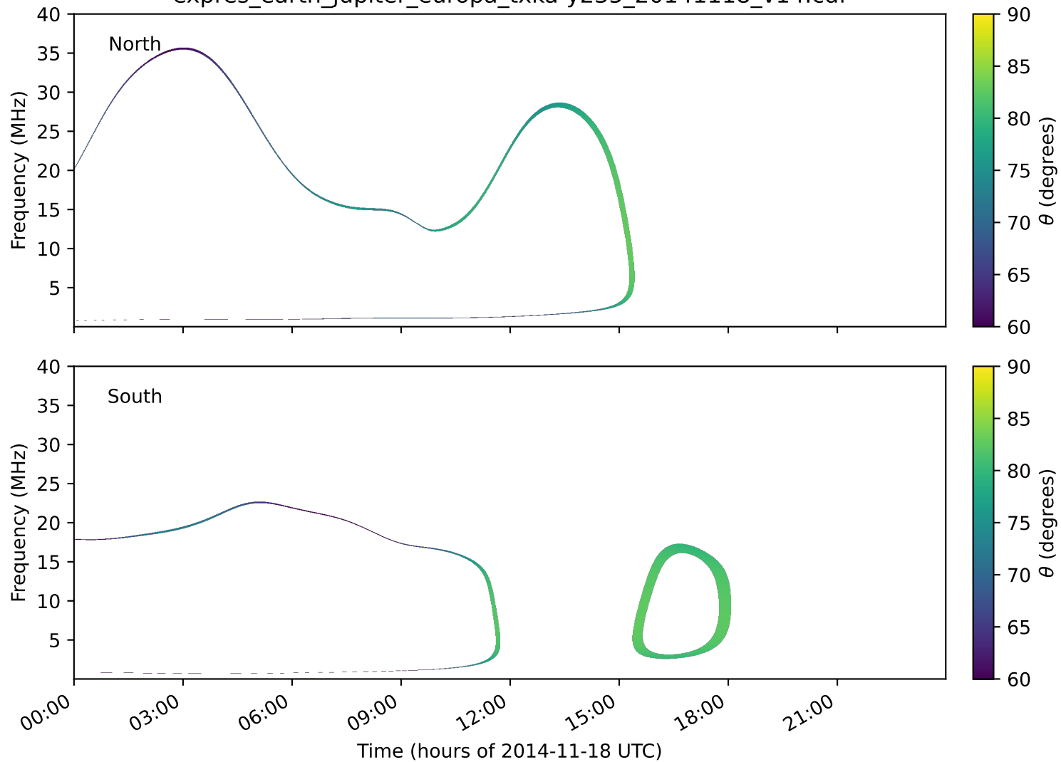
expres_earth_jupiter_europa_txka-y235_20141118_v14.cdf
