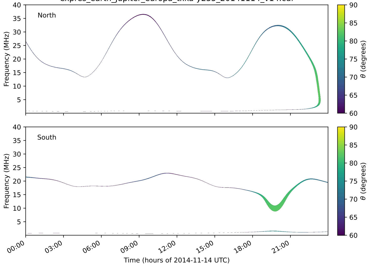
expres_earth_jupiter_europa_txka-y235_20141114_v14.cdf
