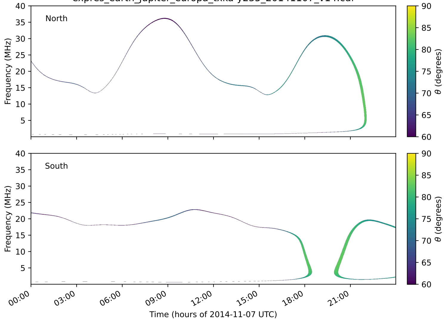
expres_earth_jupiter_europa_txka-y235_20141107_v14.cdf
