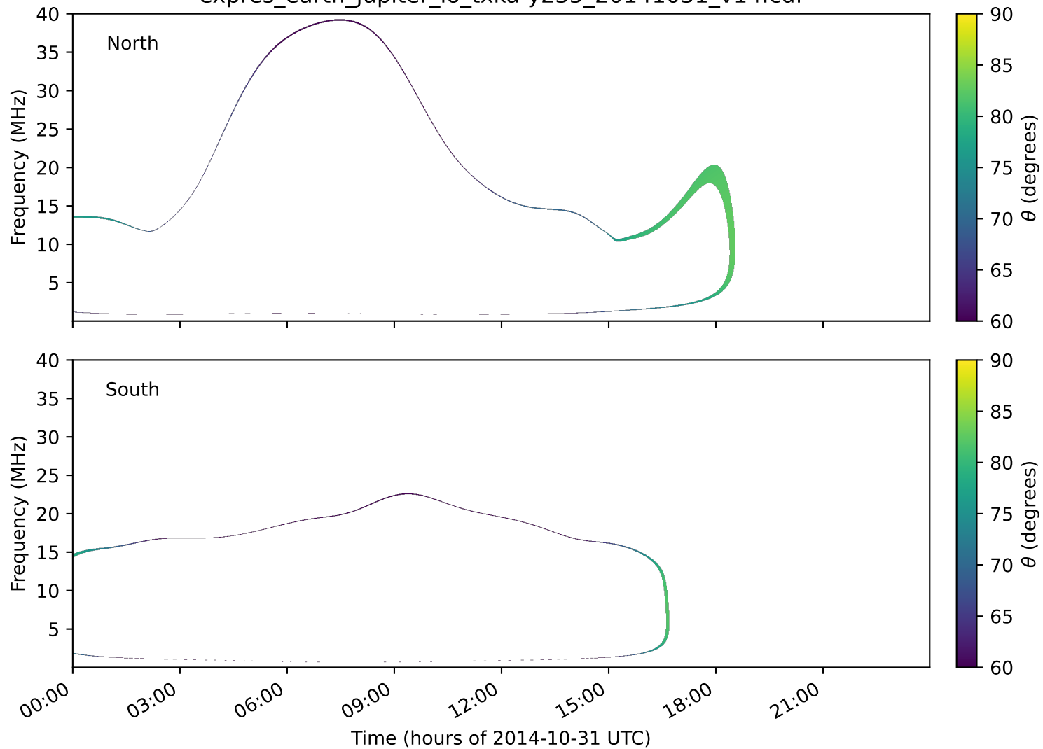
expres_earth_jupiter_io_txka-y235_20141031_v14.cdf
