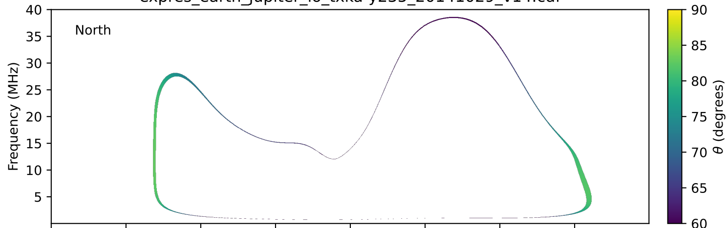
expres_earth_jupiter_io_txka-y235_20141029_v14.cdf
