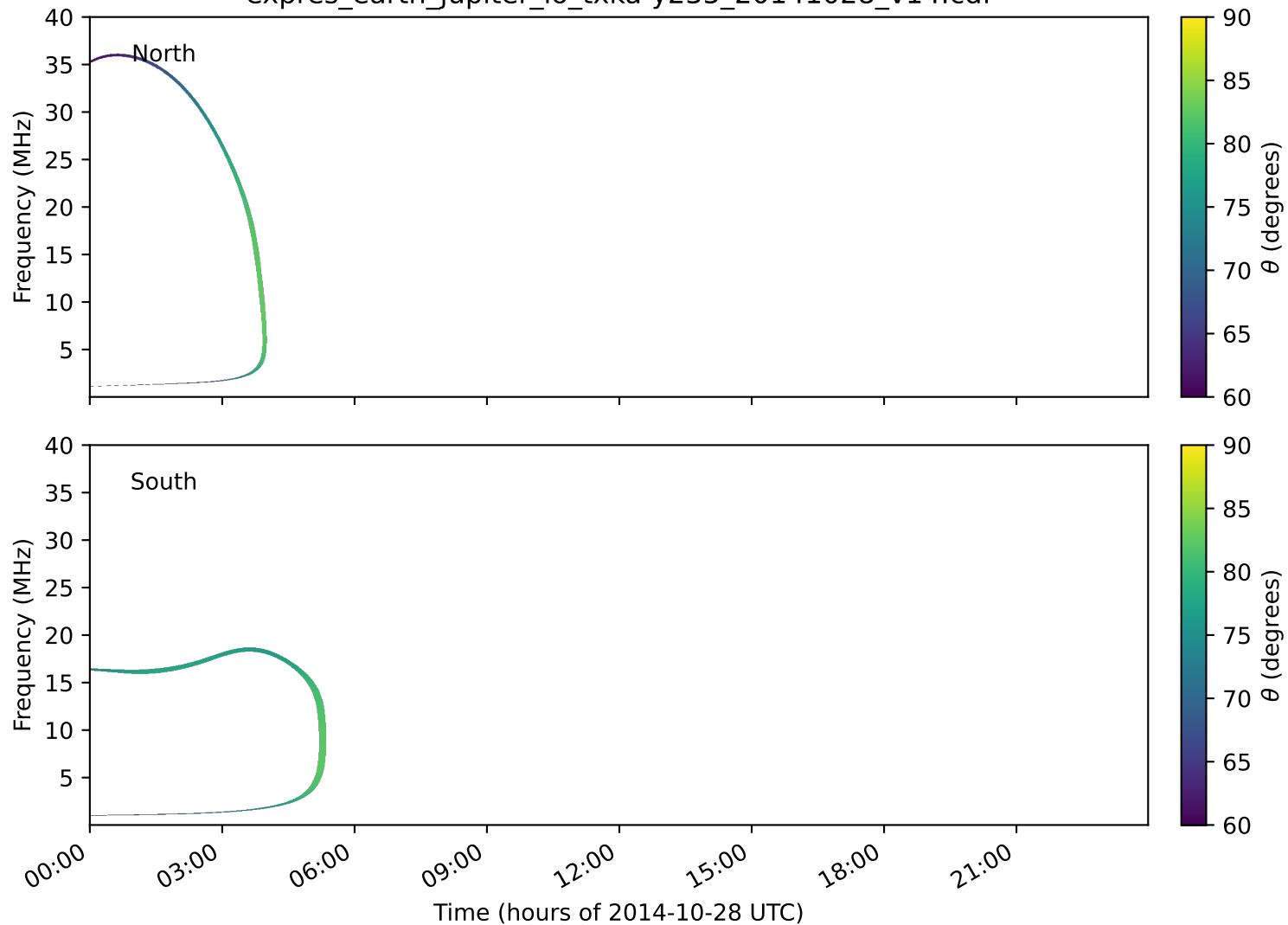
expres_earth_jupiter_io_txka-y235_20141028_v14.cdf
