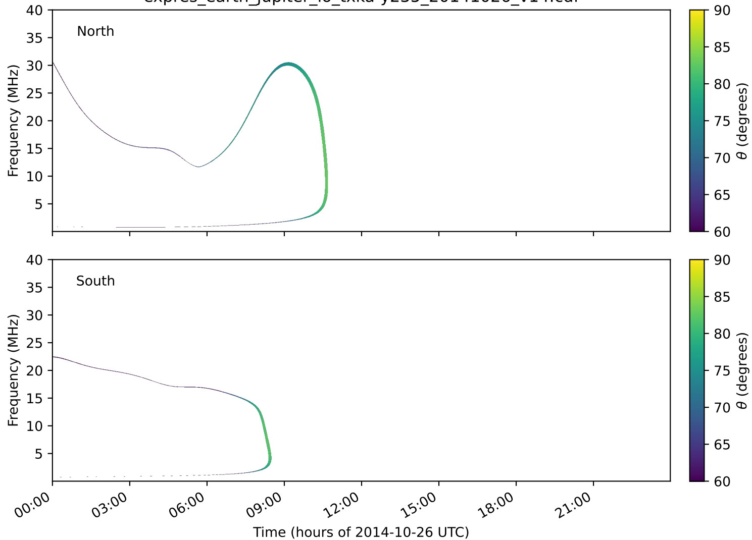
expres_earth_jupiter_io_txka-y235_20141026_v14.cdf
