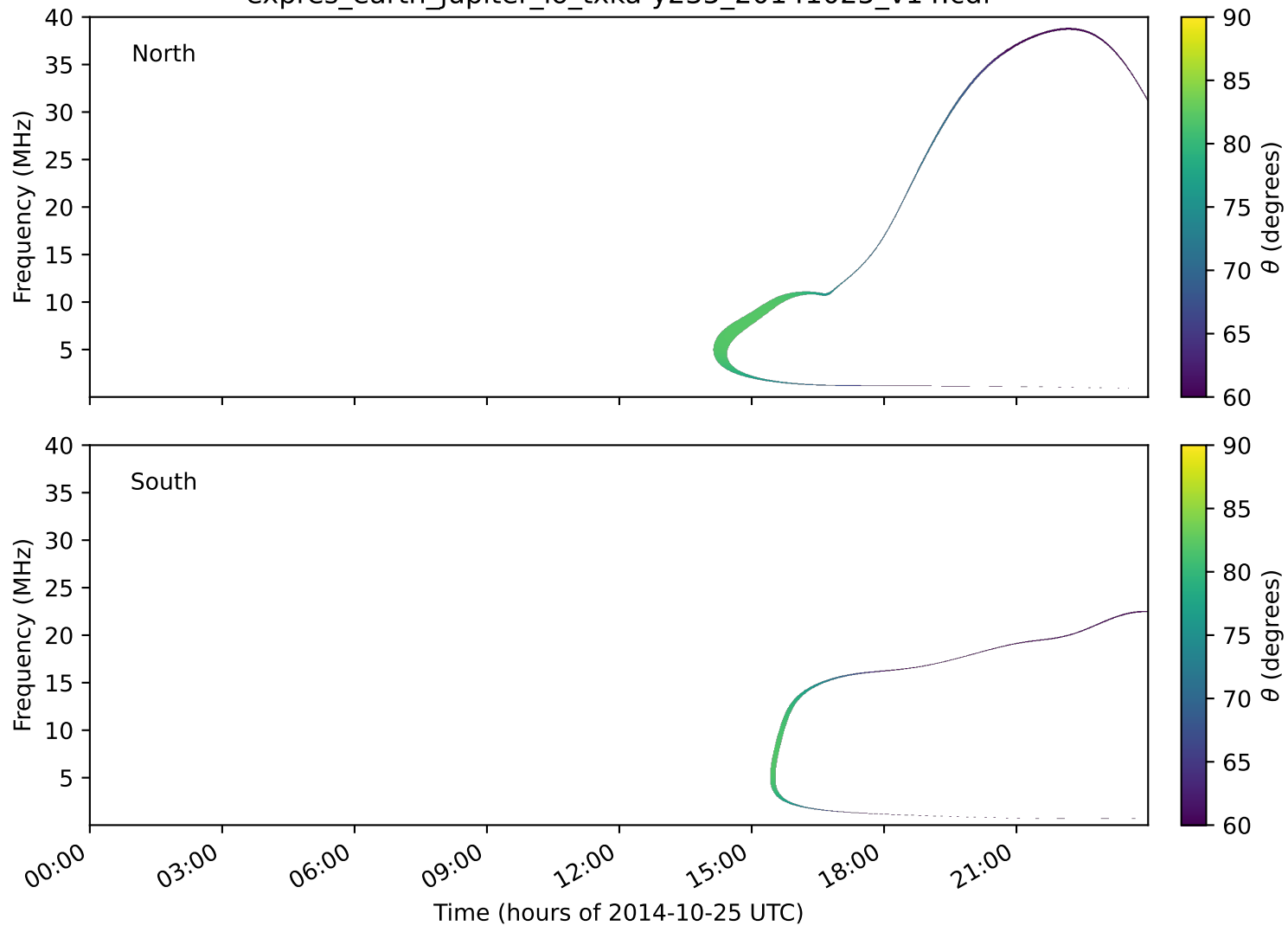
expres_earth_jupiter_io_txka-y235_20141025_v14.cdf
