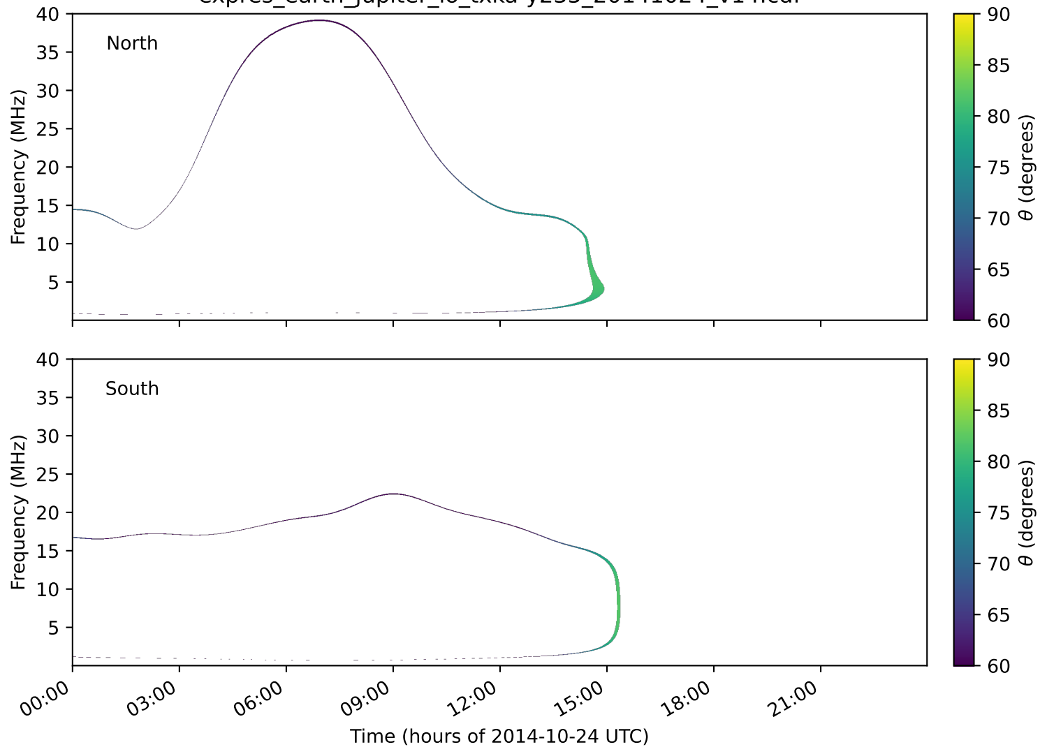
expres_earth_jupiter_io_txka-y235_20141024_v14.cdf
