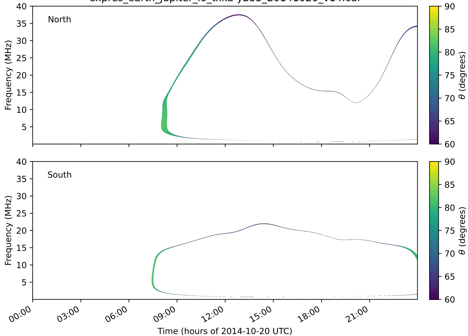
expres_earth_jupiter_io_txka-y235_20141020_v14.cdf
